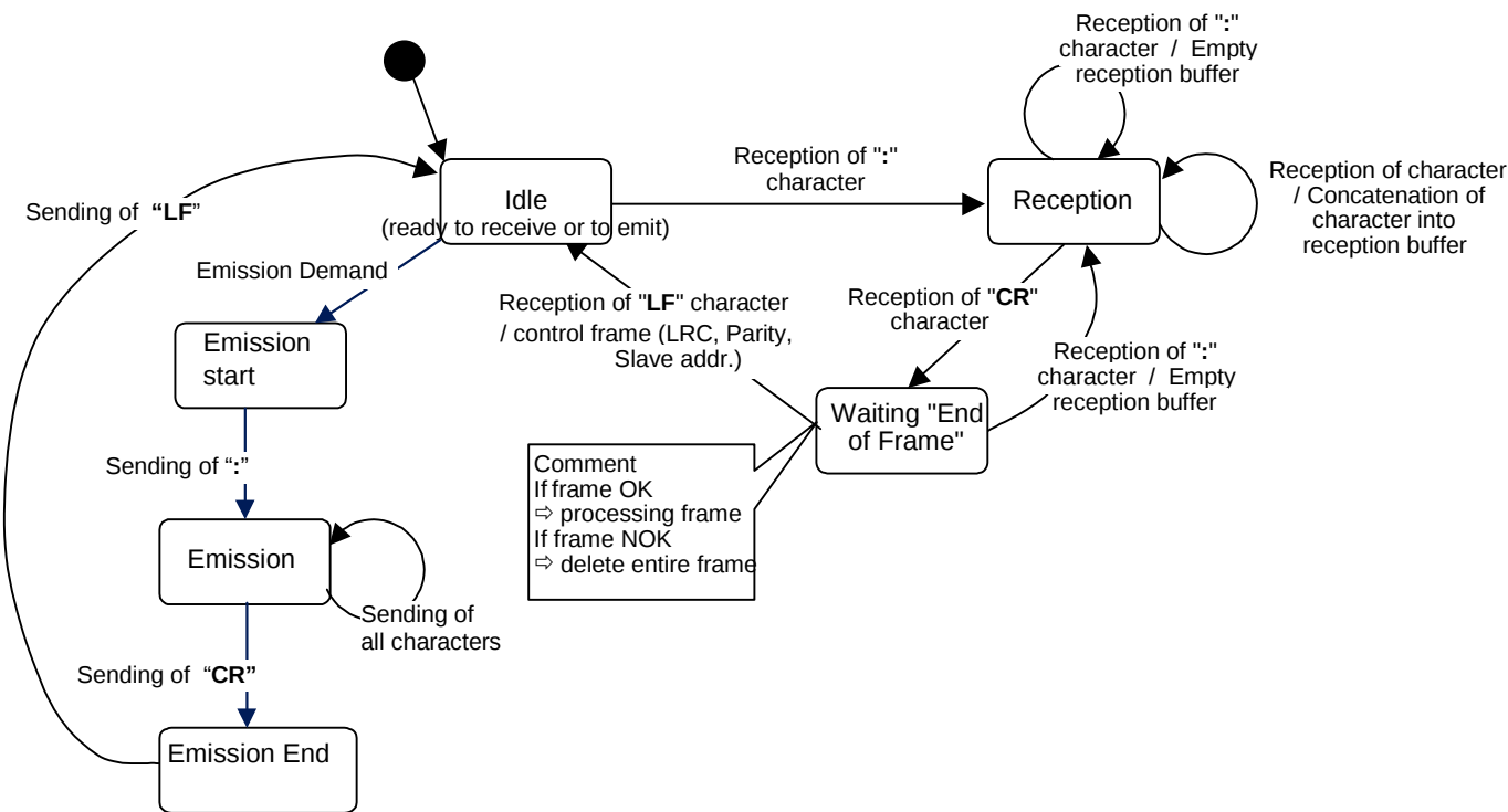
Figure 18: ASCII Transmission mode State diagram
