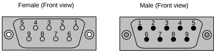
Figure 27: D-shell 9-pin connector
